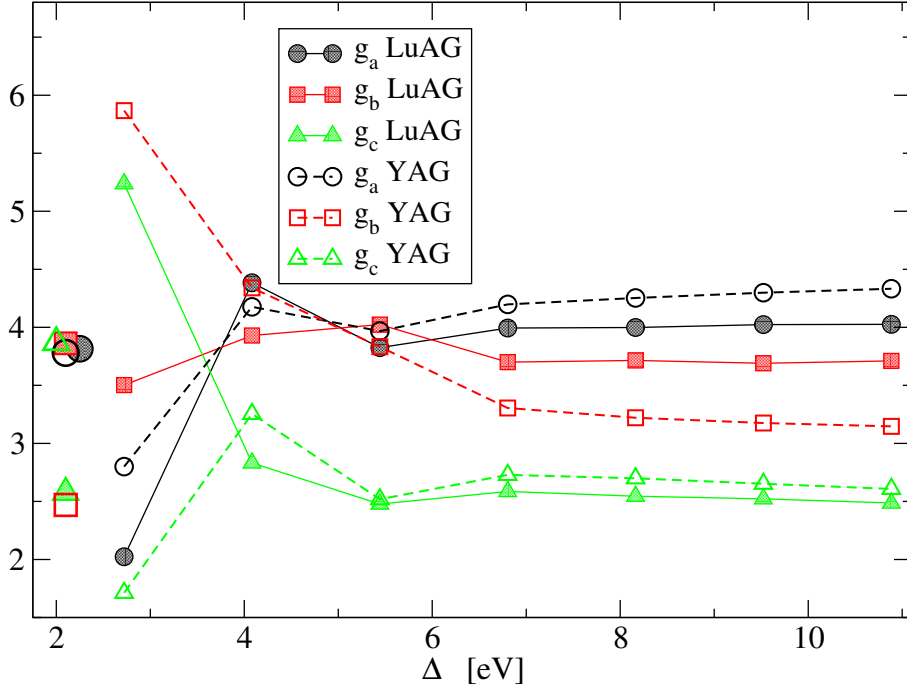
FIG. 15: Yb:YAG, LuAG. Principal components of \hat{g} as a function of the hybridization parameter \Delta . Experimental data (enlarged symbols on the left side) are taken from Refs. 29, 30.
