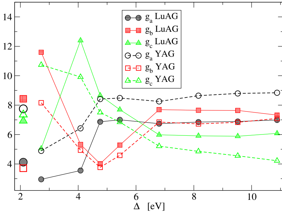
FIG. 14: Er:YAG, LuAG. Principal components of \hat{g} as a function of the hybridization parameter \Delta . Experimental data (enlarged symbols on the left side) are taken from Ref. 28.
