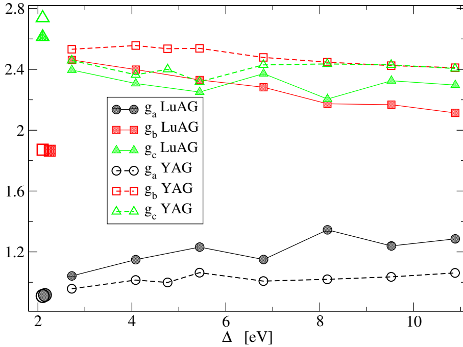
FIG. 9: Ce:YAG, LuAG. Principal components of \hat{g} as a function of the hybridization parameter \Delta . Experimental data (enlarged symbols on the left side) are taken from Refs. 25, 26.
