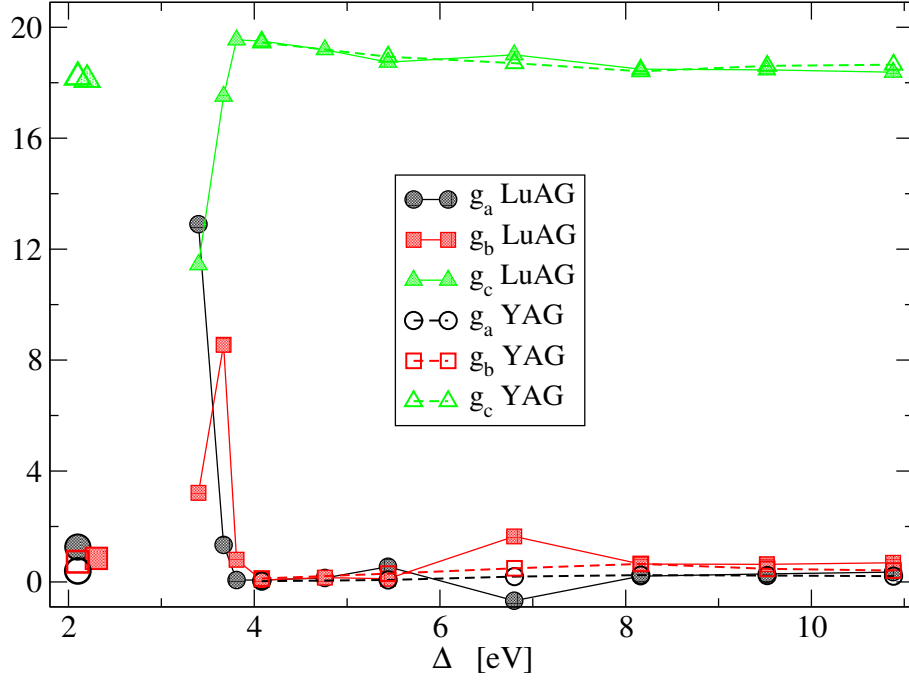
FIG. 13: Dy:YAG, LuAG. Principal components of \hat{g} as a function of the hybridization parameter \Delta . Experimental data (enlarged symbols on the left side) are taken from Ref. 28.
