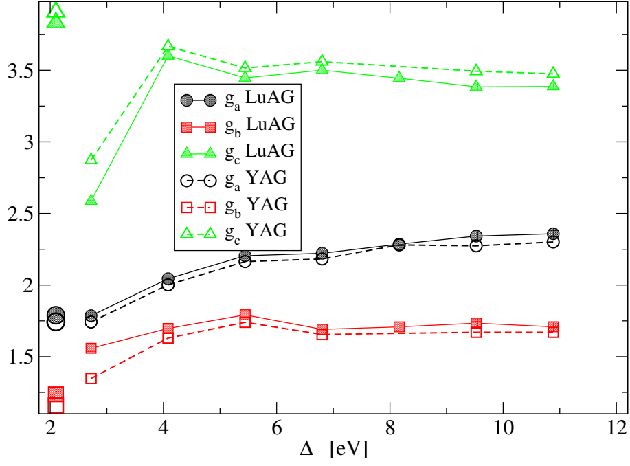
FIG. 10: Nd:YAG, LuAG. Principal components of \hat{g} as a function of the hybridization parameter \Delta . Experimental data (enlarged symbols on the left side) are taken from Refs. 24, 27.
