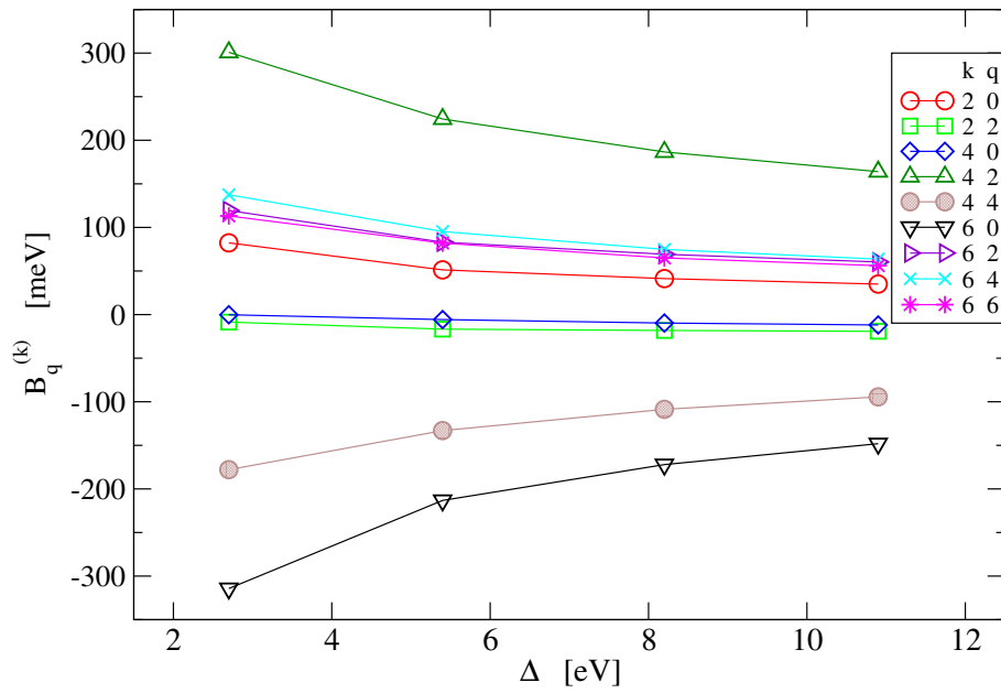
FIG. 5: Sm:YAG. CFP as a function of the hybridization parameter \Delta .
